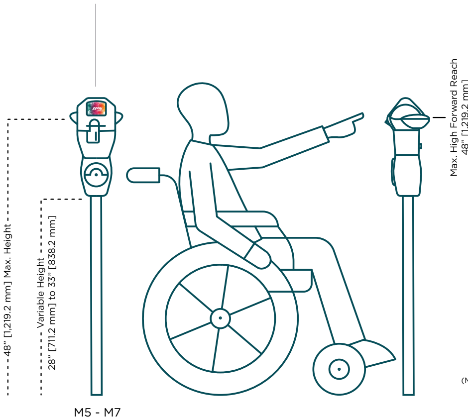
IPS Single-Space Smart Meters
